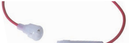
BF301 10A- 12AWG wire 6.3mm x 32mm
