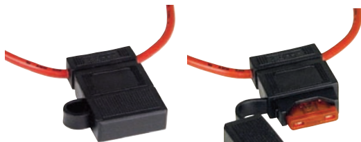
BF-351 30A- 12AWG wire water resistant ATP/ATC/ATO fuses
