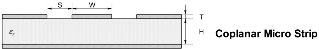
Figure 19: Coplanar micro-strip dimension specification
