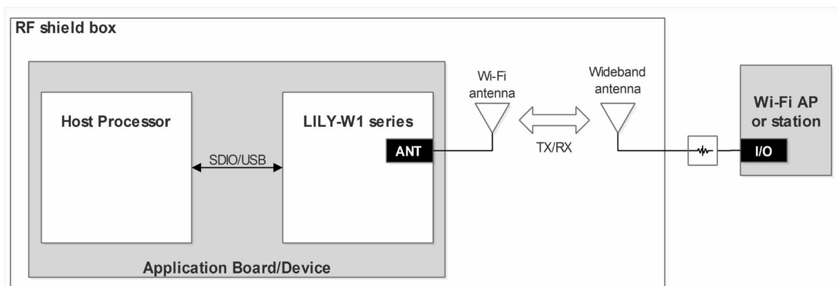
Figure 15: Setup with RF shield box and standard Wi-Fi/Bluetooth devices for radiated tests
