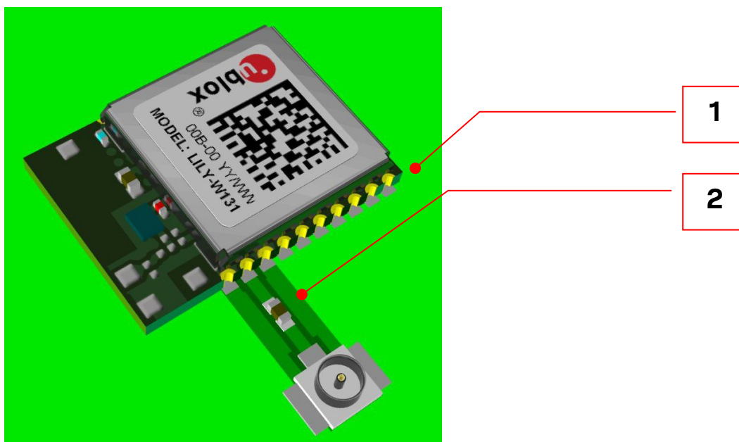
Figure 17: Antenna Reference design embedded in a host carrier PCB
