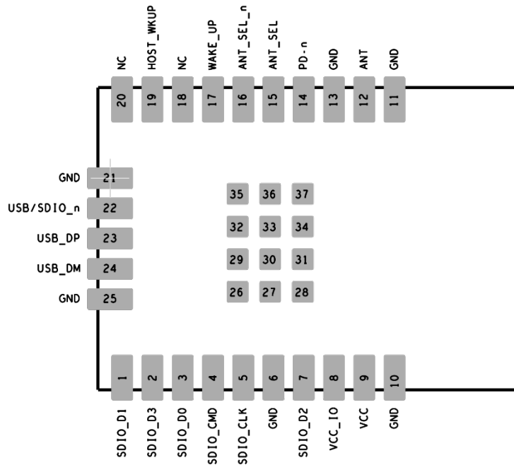
Figure 2: LILY-W1 pin assignment (top view)
