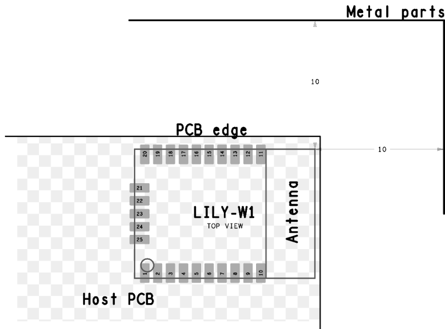
Figure 7: LILY-W132 PCB placement recommendation (dimensions are in mm)
