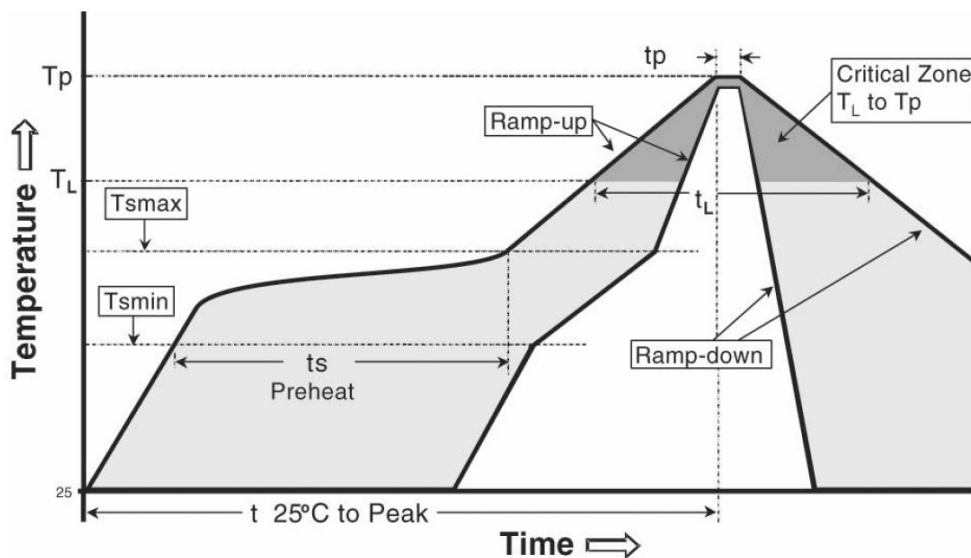
Figure 12: Reflow profile
