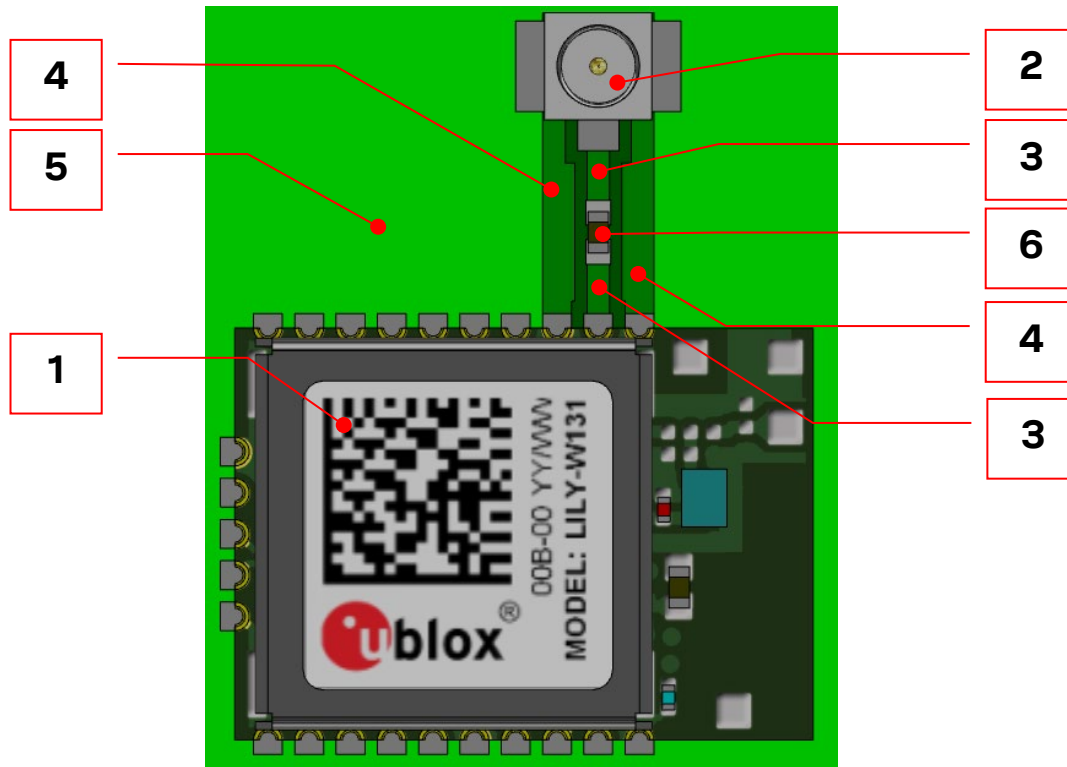
Figure 18: LILY-W131 antenna reference design
