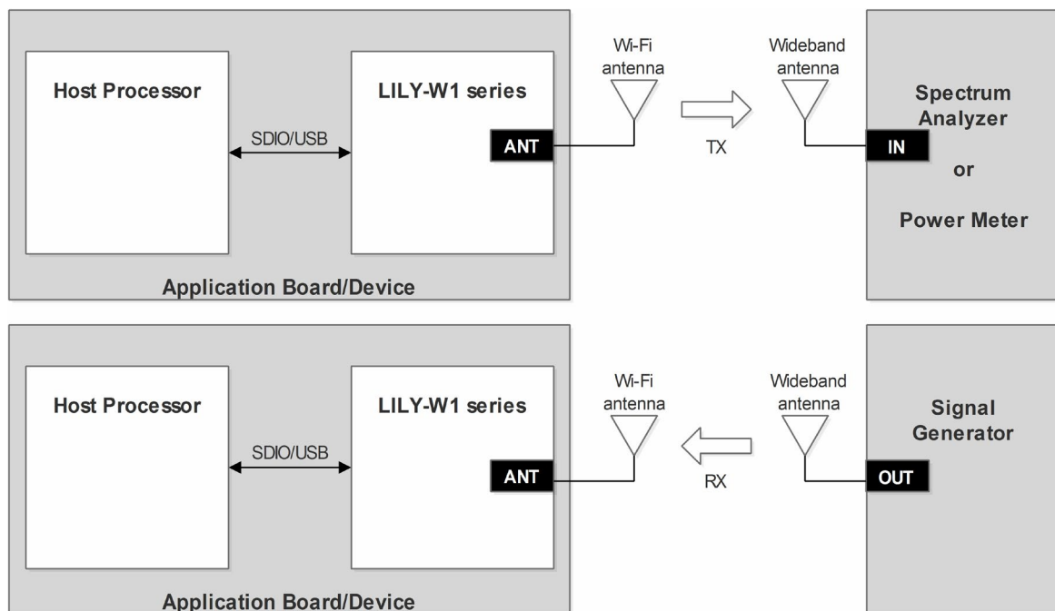
Figure 16: Setup with spectrum analyzer or power meter and signal generator for radiated measurement
