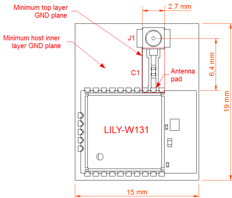
Figure 20: Mechanical dimensions of EVK-LILY-W131
