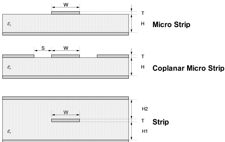
Figure 4: Transmission line trace design
