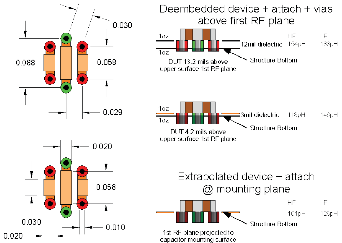
Figure 2, X2Y® Recommended Layouts, and Bypass Measurements
