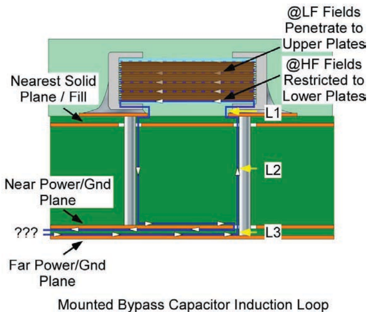
Figure 1, Bypass Capacitor Mounted Inductance
